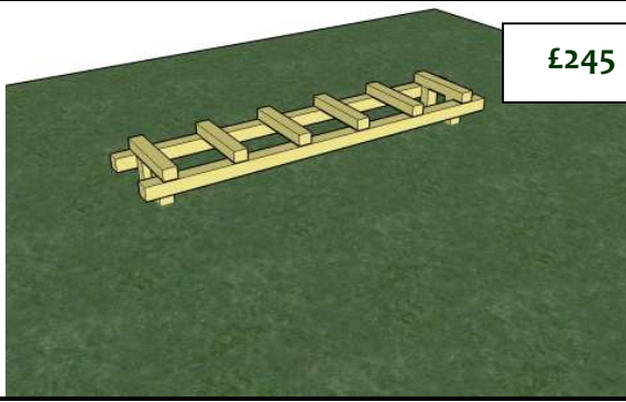
Ladder Walk; 100mm x 100mm cross pieces on 2m long 100mm x 100mm frame. Nominal height 350mm above ground.
