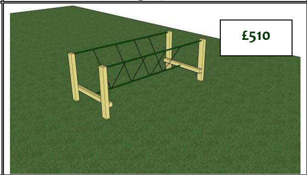
Monkey Bridge; steel cored rope traverse fixed between 150mm x 100mm end pieces. Overall length 2.5m, width 2m.
