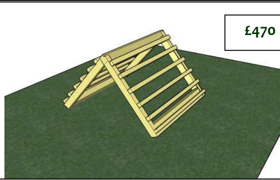
Ladder wall; 1.2m high to apex, 2m width. Each face made up of 100mm x 100mm cross bars on 150mm x 100mm frame.
