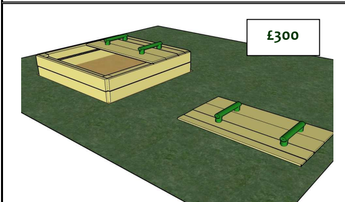
Sandbox with removable cover; 100mm x 100mm frame, 150mm x 50mm planking. Complete with lift-off 2 part lid with handles and membrane base. Overall size 1.5m x 1.5m. Larger sizes available.
